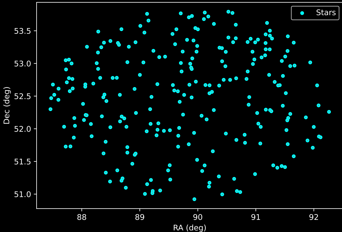
APOGEE DR17 Field: [109-08] Proper Motion Vectors for Gaia Star Field (n= 238)
