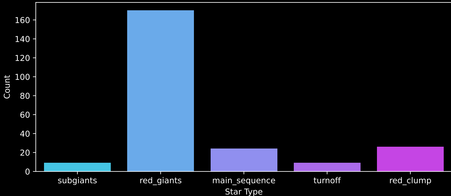
APOGEE DR17 Field: [109-08] Count plot of Star Type
