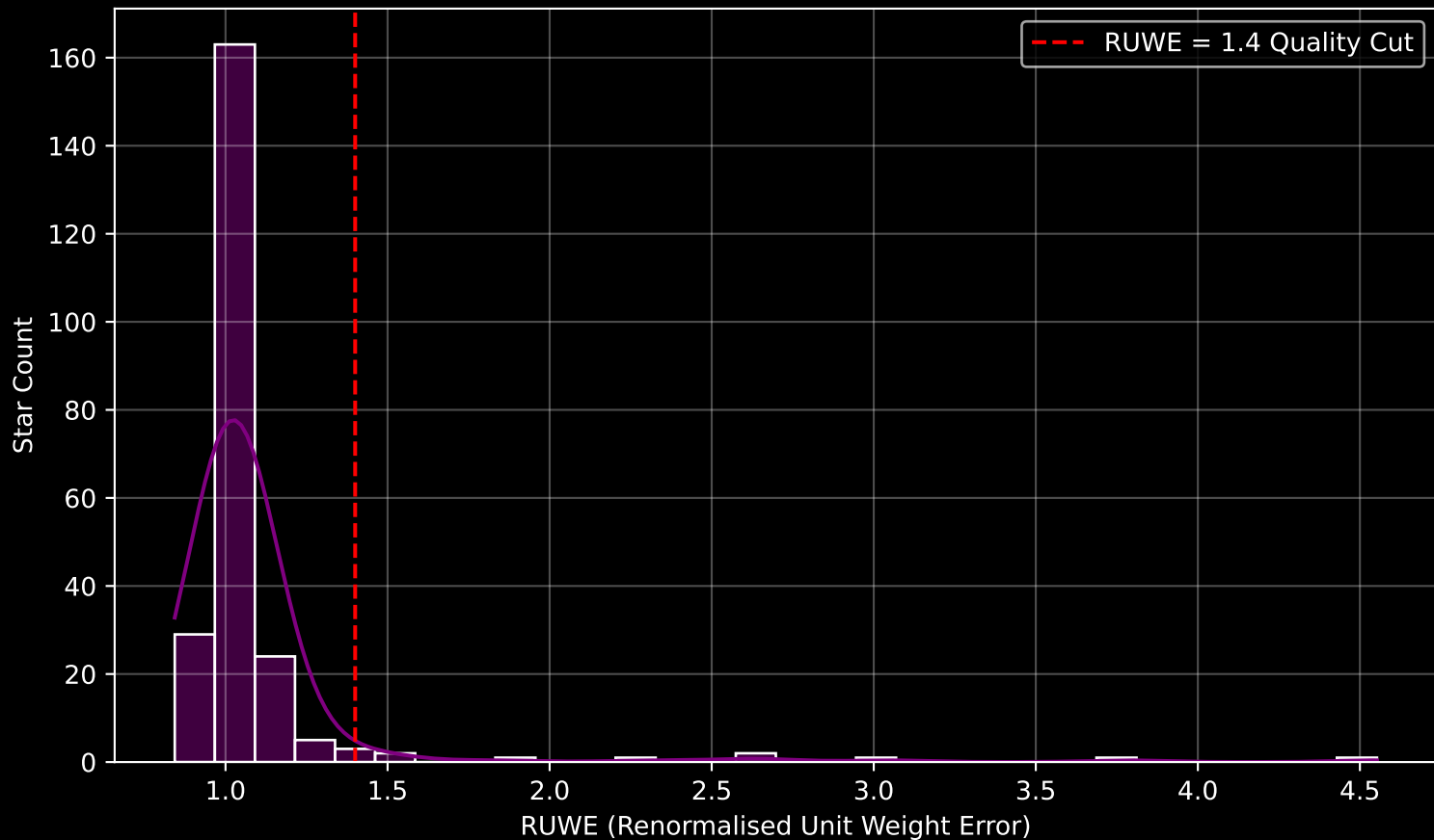
GAPOGEE DR17 Field [109-08] RUWE Distribution (n= 233)
