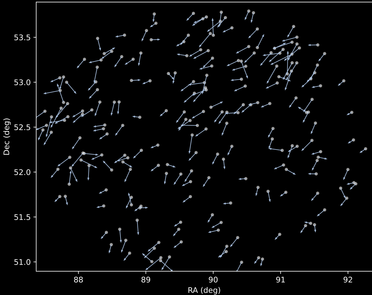
APOGEE DR17 Cluster 1 Proper Motion Vectors (n=216)
