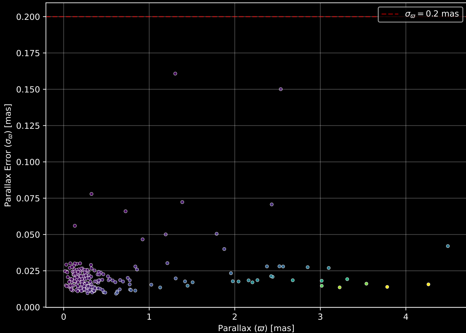
APOGEE DR17 Field: [109-08] Parallax Quality (n= 238)
