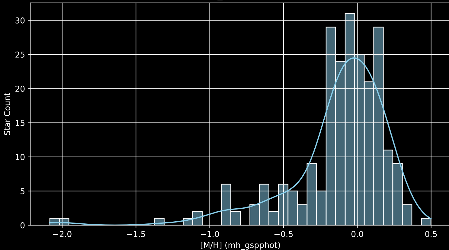
APOGEE DR17 Field: [109-08 [M/H] (mh_gspphot) (n= 236)
