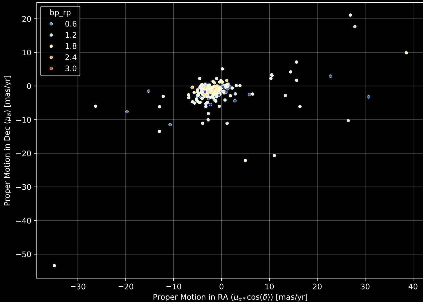
APOGEE DR17 Field: [109-08] Proper Motion Diagram (n= 238)
