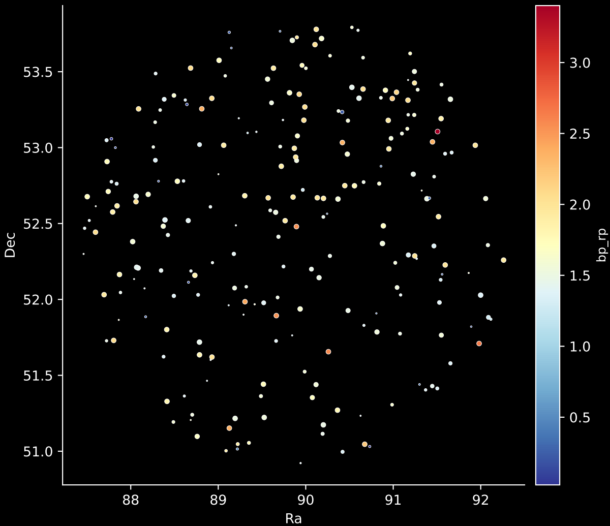
APOGEE DR17 Field: [109-08] Stars: 238
